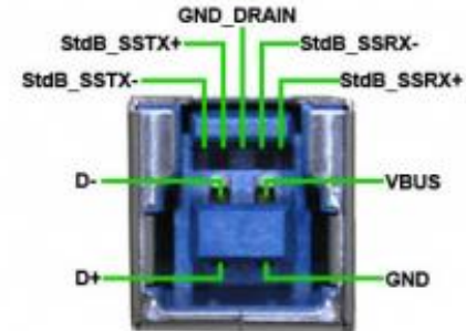
SuperSpeed standard B plug pinout
